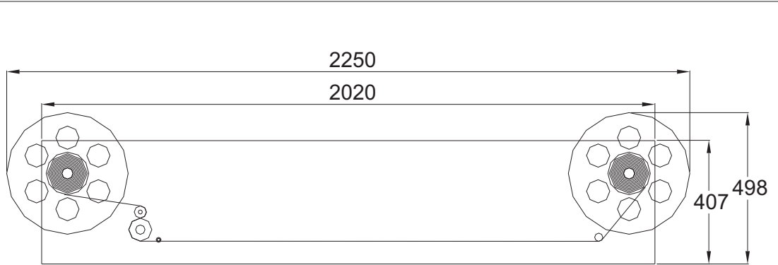
High Speed Label Roll Winding and Counting Machine :Spl with extended Web Length
