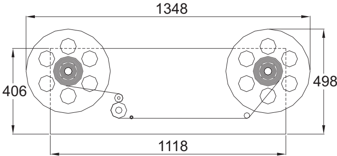
Label Roll Winding and Counting Machine : Standard
